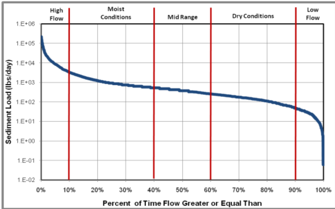
Figure C-6: Accotink Creek Sediment Load Duration Curve
