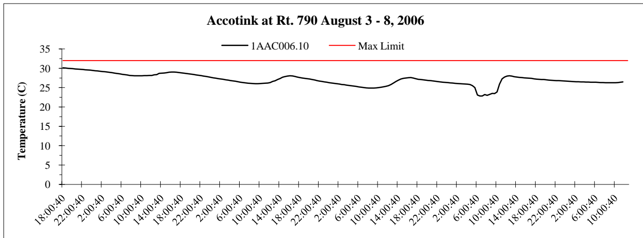
Figure 3-27: Continuous Ambient Monitoring of Temperature in Accotink Creek in August of 2006
