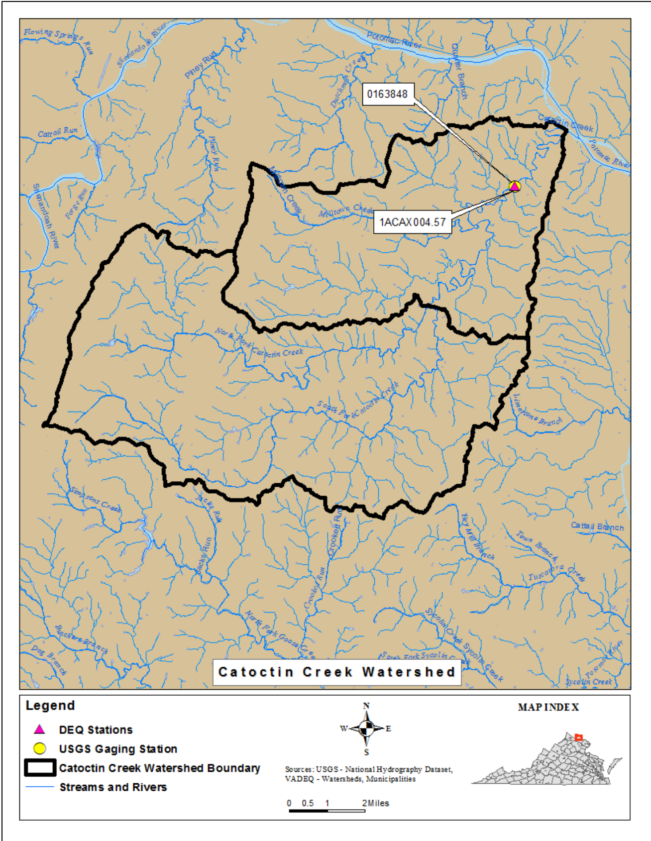
Figure 5-3: Catoctin Creek Watershed and Monitoring Stations
