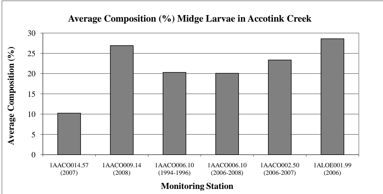
Figure 3-4: Average Percent Composition of Midge Larvae in the Accotink Creek Watershed
