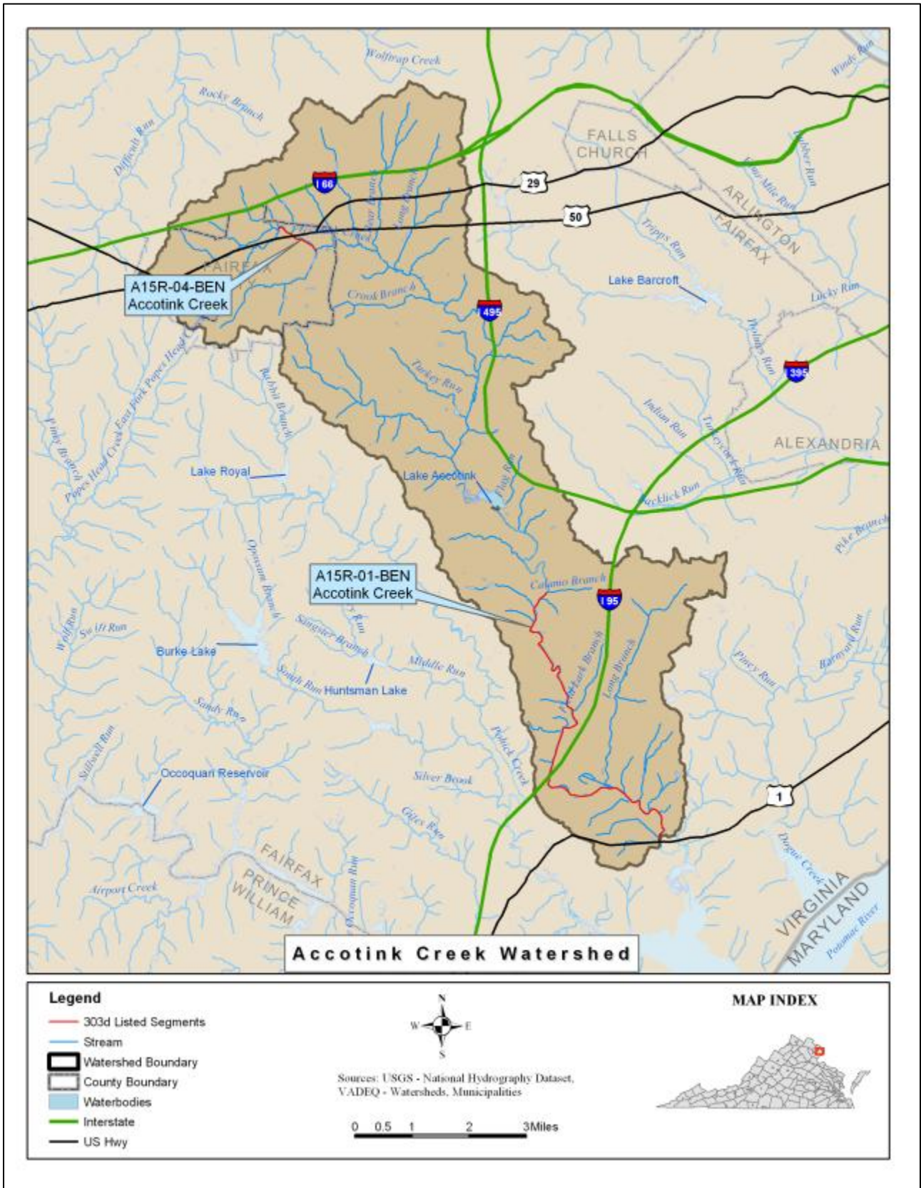
Figure 1-1: Accotink Creek Benthic Impaired Segments and Delineated Watershed
