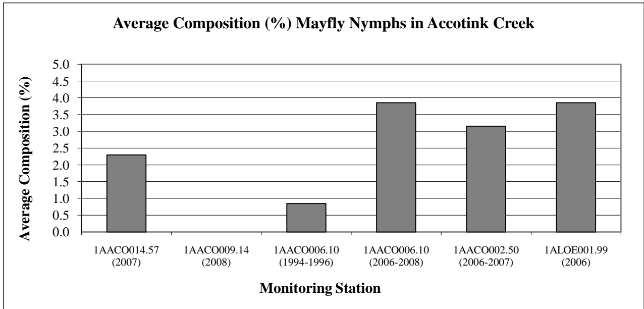
Figure 3-3: Average Percent Composition of Mayfly Nymphs in the Accotink Creek Watershed
