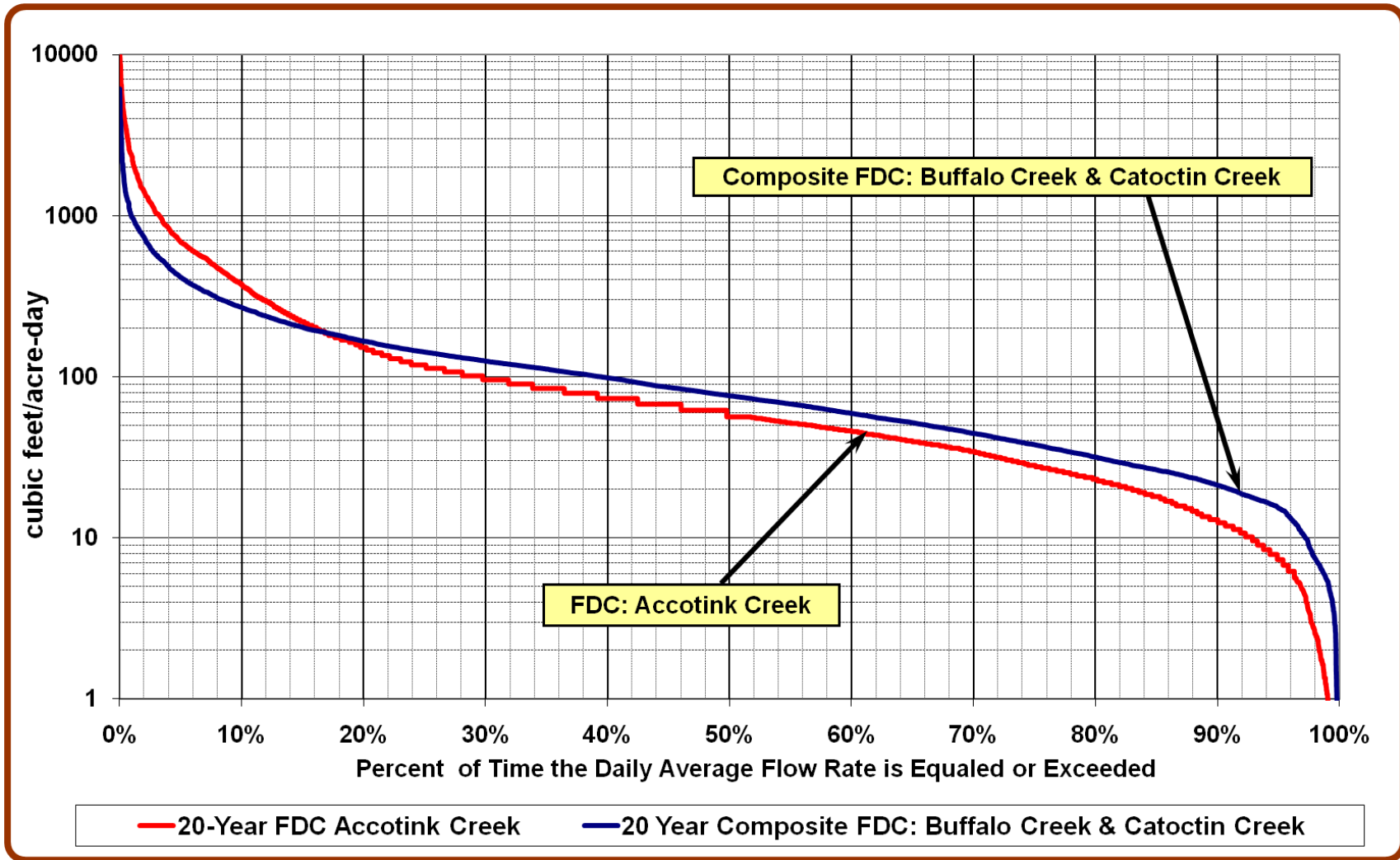
Figure 5-4. Accotink Creek FDC and Composite FDC (Buffalo Creek & Catoctin Creek) using 20-year Flow Record (11/1989 – 11/2009)
