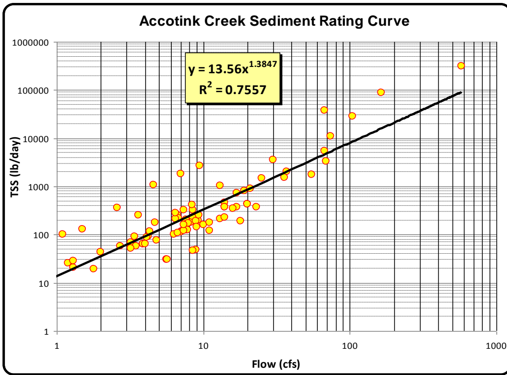
Figure 4-1: Accotink Creek Sediment Rating Curve
