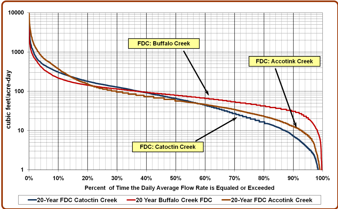
Figure 5-5. Catoctin Creek, Buffalo Creek and Accotink Creek FDCs using 20-year Flow Record (11/1989 – 11/2009)
