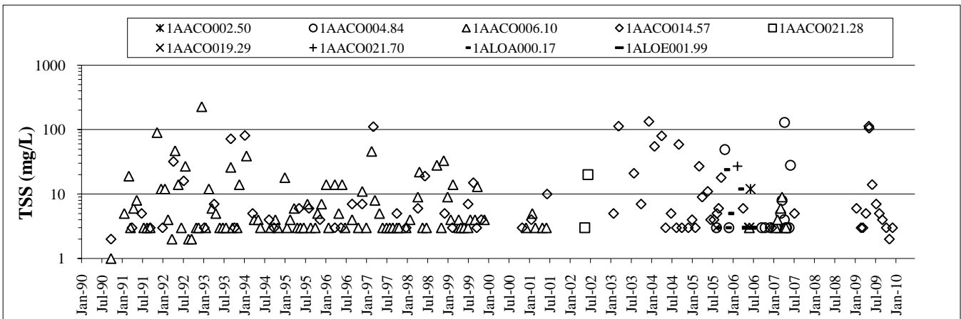
Figure 3-20: Ambient TSS in the Accotink Creek Watershed
