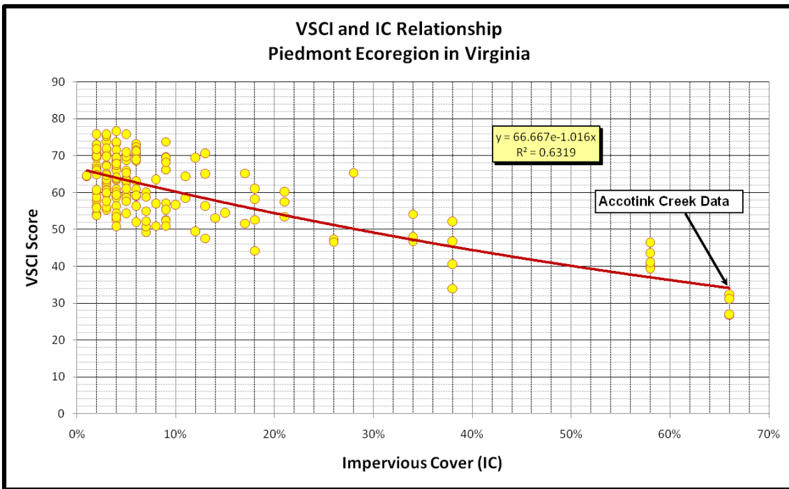
Figure C-7: VSCI and IC Relationship for the Piedmont Ecoregion in Virginia
