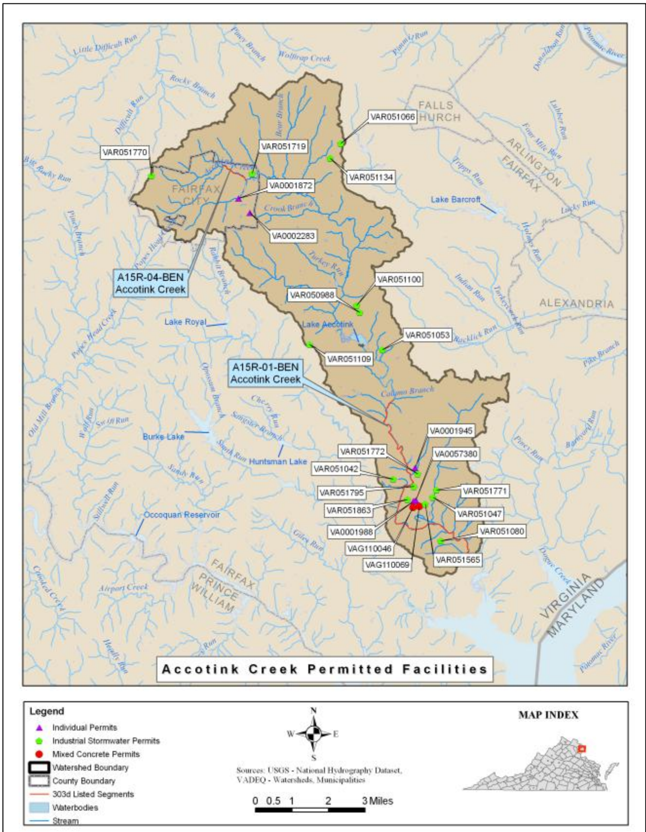
Figure 2-4: Location of Permitted Facilities in the Accotink Creek Watershed
