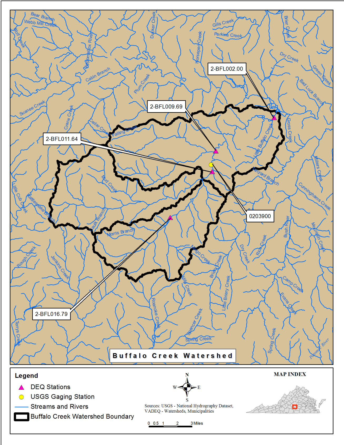
Figure 5-2: Buffalo Creek Watershed and Monitoring Stations
