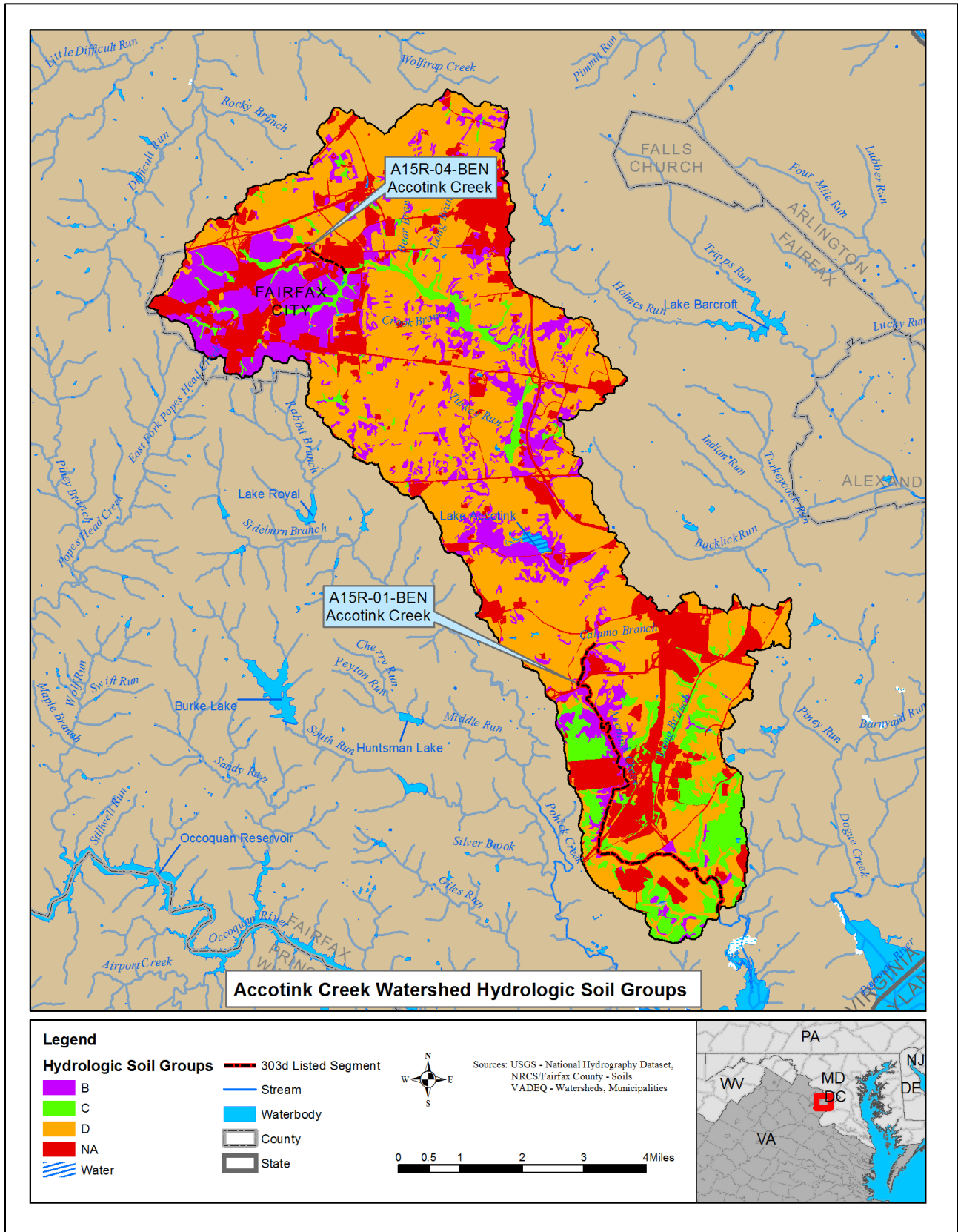
Figure 2-1: Hydrologic Soil Group Distribution in the Accotink Creek Watershed
